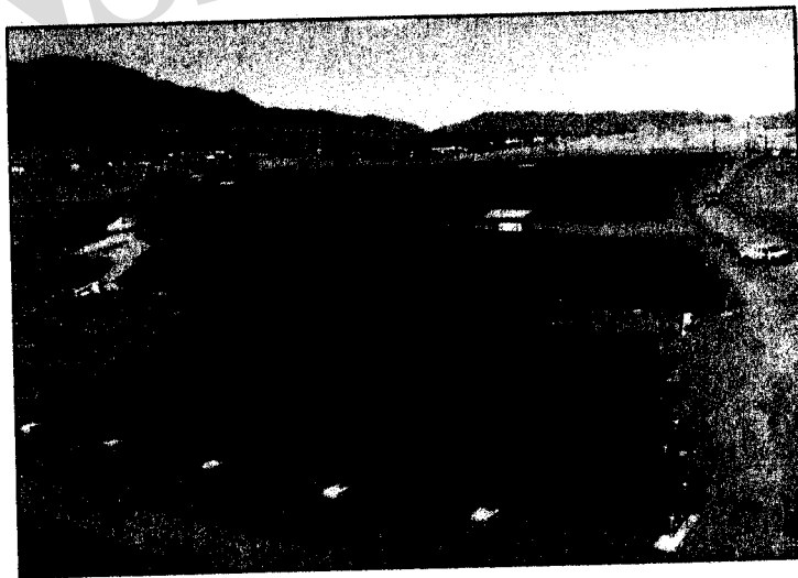
At Fort Carson, Colo., the Army partnered with a local energy provider in an enhanced-use lease. The energy provider built a photovoltaic solar array on top of a closed landfill. That site now provides energy to some 540 homes. U.S. Army photo.
